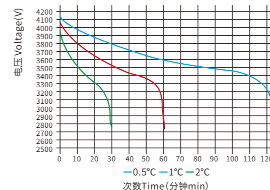
Discharge characteristics
